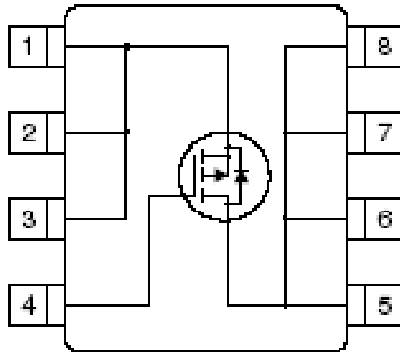
P-Channel MOS FET (1 device built-in)
