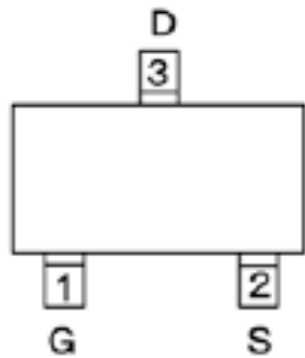
SOT-23 (TOP VIEW)
