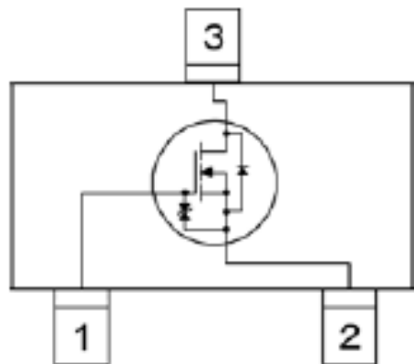
N-channel MOSFET (1 device built-in)
