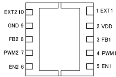
USP-10 (BOTTOM VIEW)
