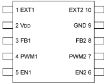
MSOP-10 (TOP VIEW)
