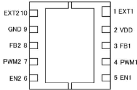
USP-10 (BOTTOM VIEW)
