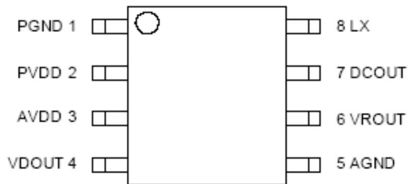
SOP-8 (TOP VIEW)
