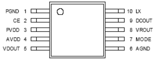
MSOP-10 (TOP VIEW)
