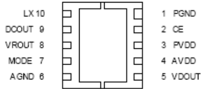
MSOP-10 (TOP VIEW)
