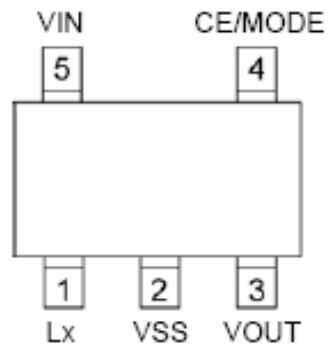
SOT-25 (TOP VIEW)
