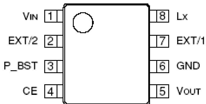
SOP-8 (TOP VIEW)
