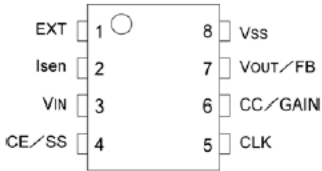
MSOP-8A (TOP VIEW)
