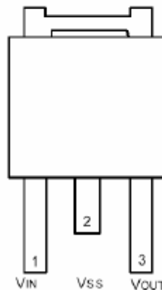
TO-252 (TOP VIEW)
