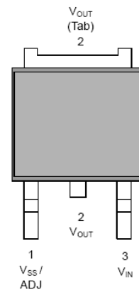
TO-252 (TOP VIEW)
