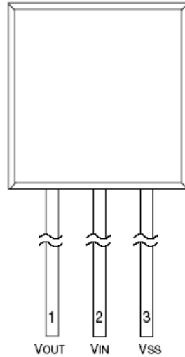
TO-92 (T Type) (TOP VIEW)
