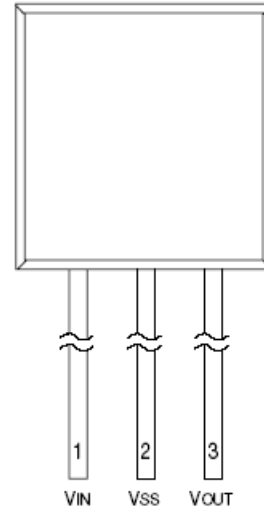
TO-92 (L Type) (TOP VIEW)
