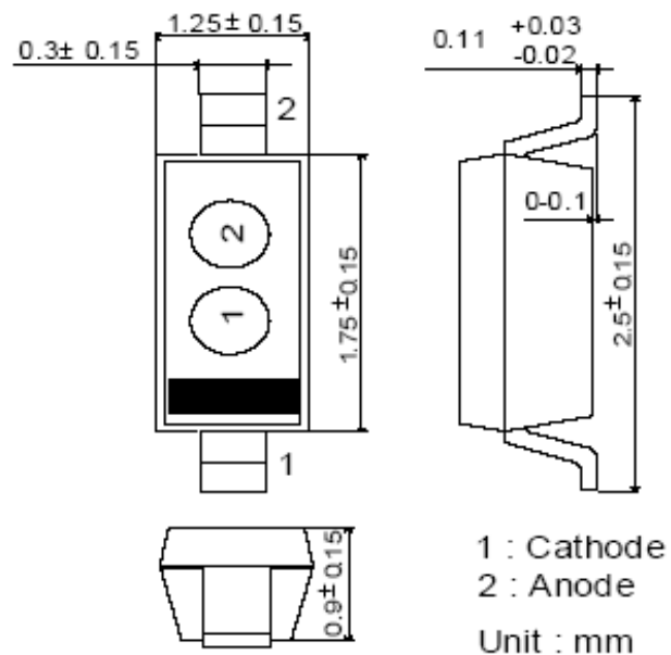
SOD-323
